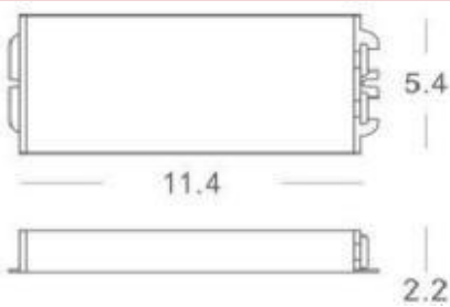
Dimension unit:cm
