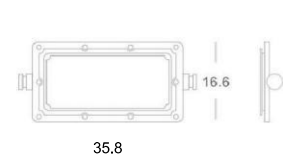
Dimenstion unit:cm
