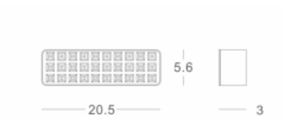
Dimenstion unit:cm
