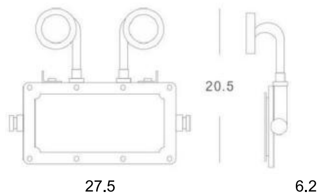
Dimenstion unit:cm
