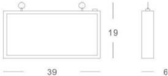
Dimenstion unit:cm
